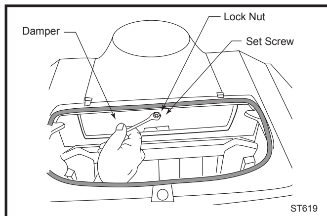
Fig. 35 When the damper's gasket becomes compressed after prolonged use, the damper should be adjusted to regain a tight seal.
