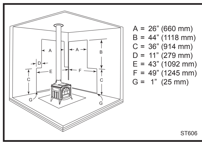
Fig. 20 A top-exit stove with reduced rear and side wall clearances. Note that rear wall shield must extend completely to corner.
