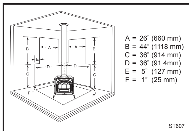
Fig. 21 A top-exit stove with reduced rear and side wall clearance. Wall shields must meet at corner.
