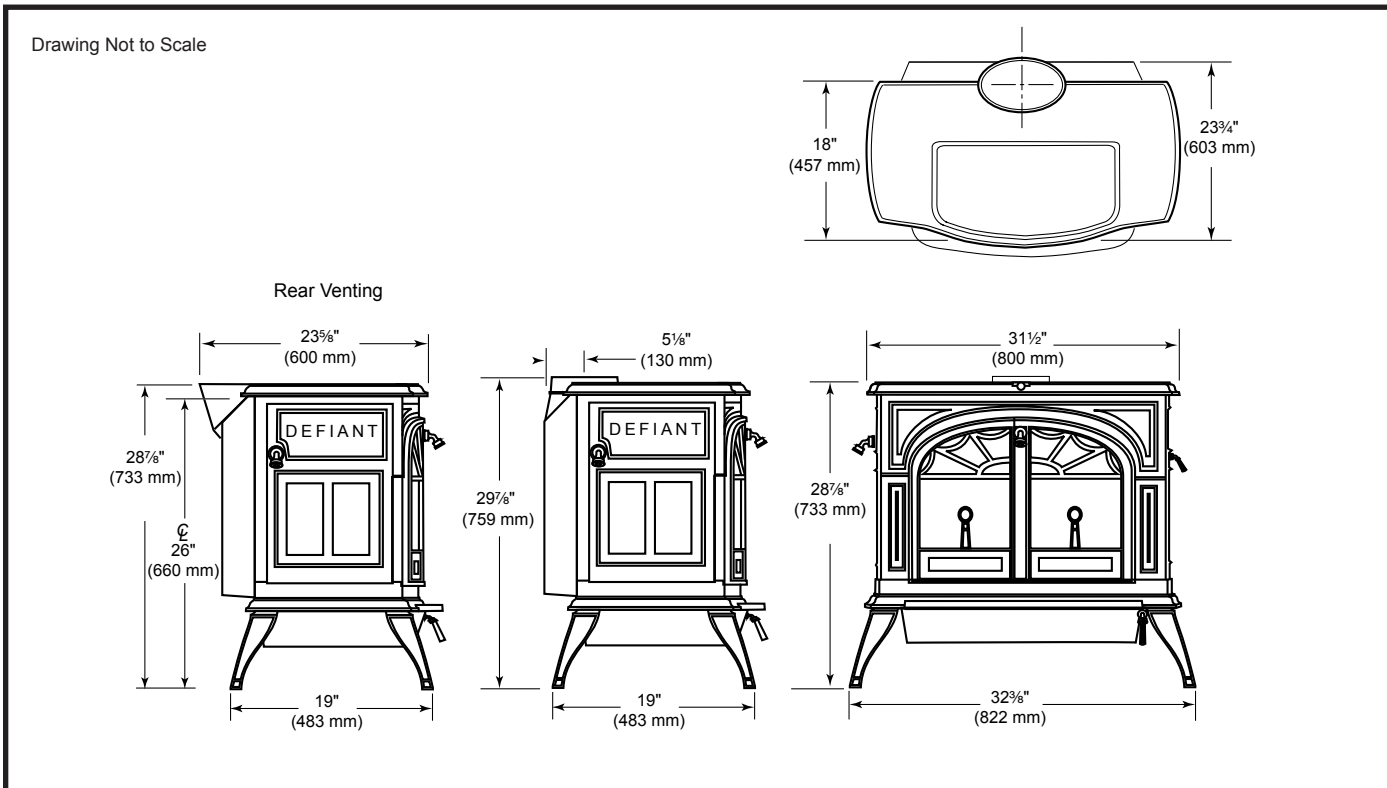
Fig. 1 Defiant NC dimensions.
