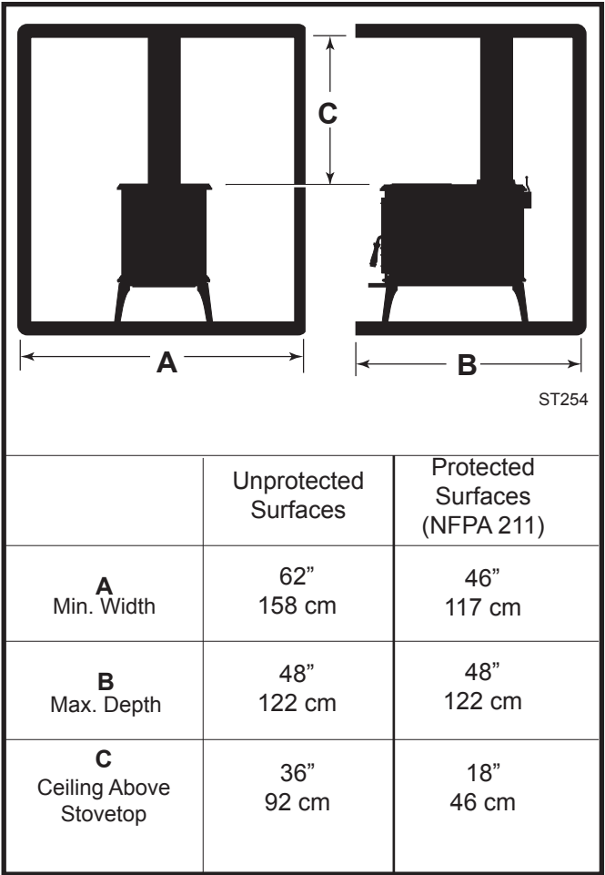
Fig. 21 Alcove Specifications.
